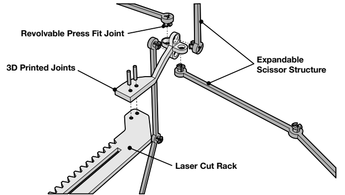
Fig. 5. The assembly of the PufferBot.
