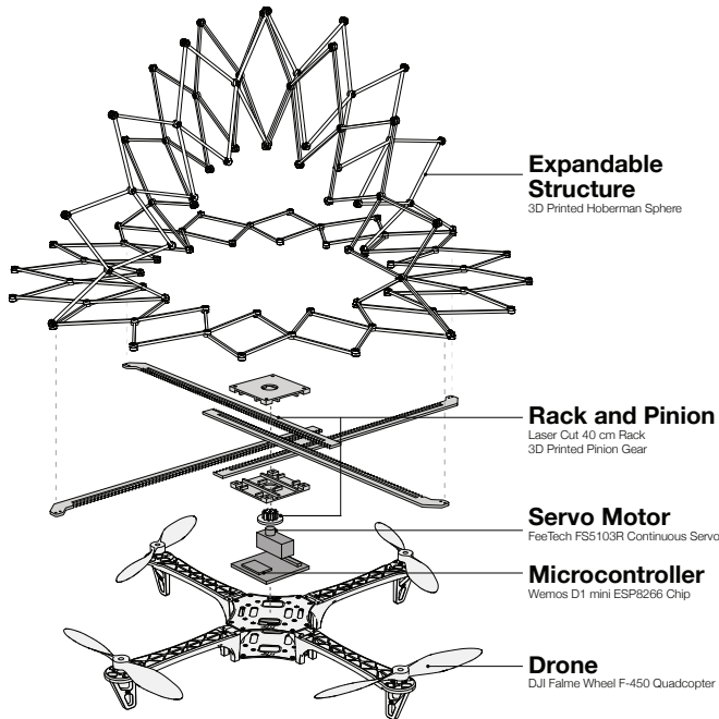
Fig. 4. PufferBot parts
