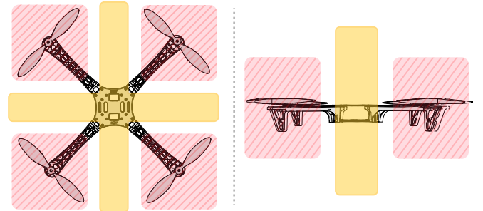
Fig. 2. Yellow area shows the two geometric planes which can be used for an actuator of expandable structure
